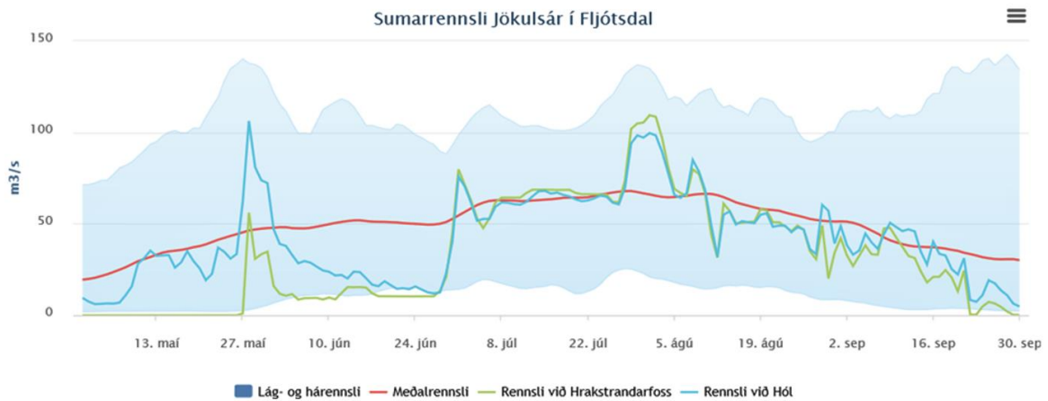
Figure 4. Summer water flow of Jökulsá í Fljótsdal river 2018
