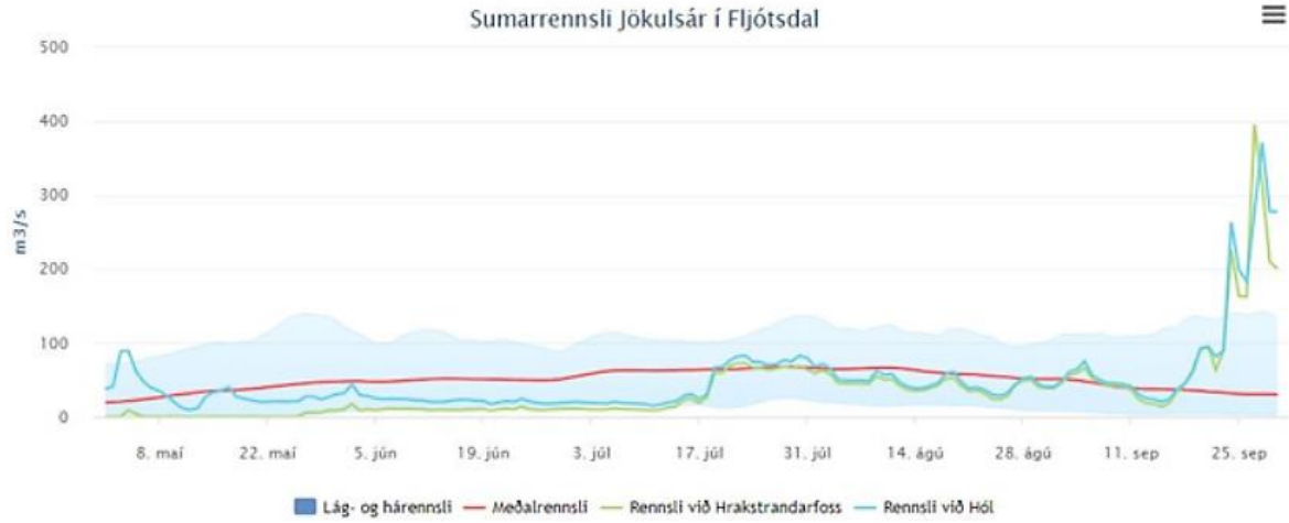
Figure 5. Summer water flow of Jökulsá í Fljótsdal river 2017
