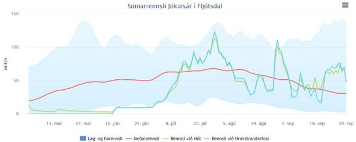
Figure 3. Summer water flow of Jökulsá í Fljótsdal river 2019
