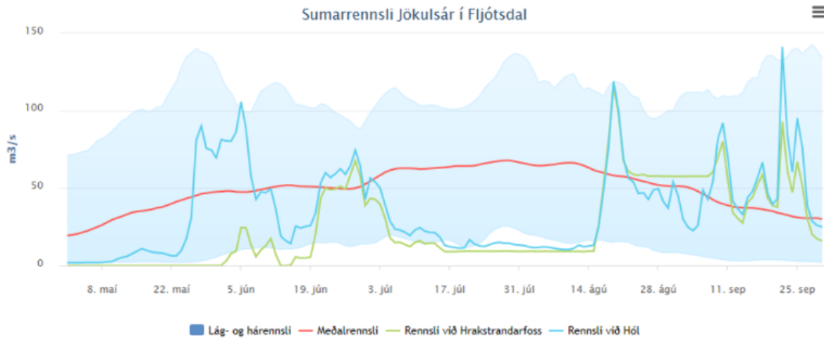
Figure 6. Summer water flow of Jökulsá í Fljótsdal river 2016
