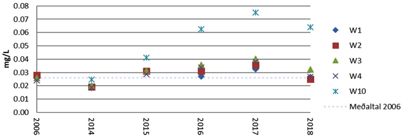
Figure 2. Annual average fluorine (mg/L) content measured in samples from rivers and Grænavatn lake in Reyðarfjörður 2004-2018.
