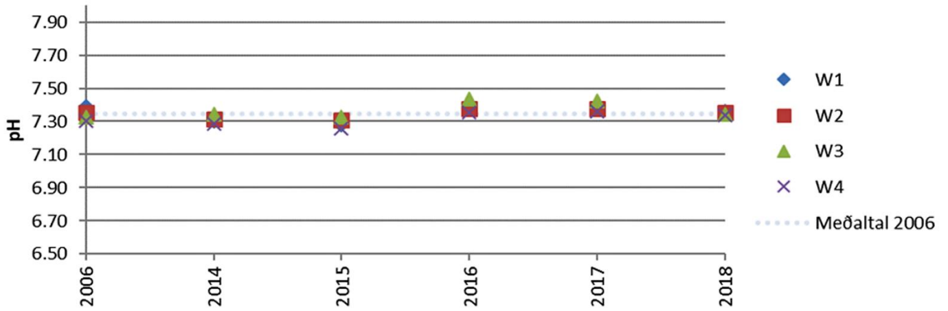
Figure 1. Annual average acidity (pH) measured in samples from rivers in Reyðarfjörður 2004-2018.
